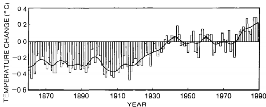
Figure 11: Global-mean combined land-air and sea-surface temperatures, 1861–1989, relative to the average for 1951–80
